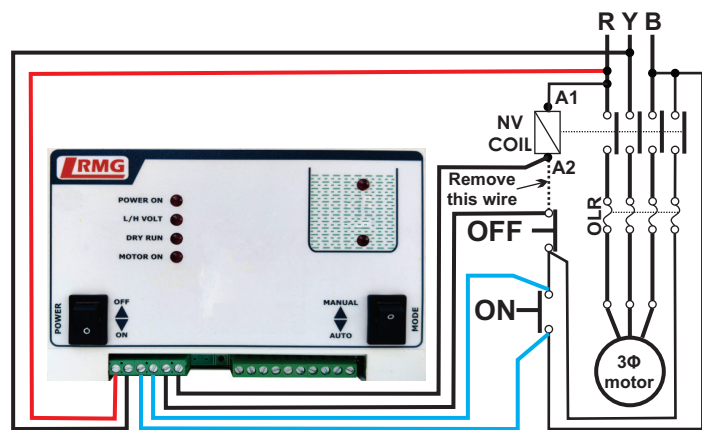
Figure2: 3Φ Starter
